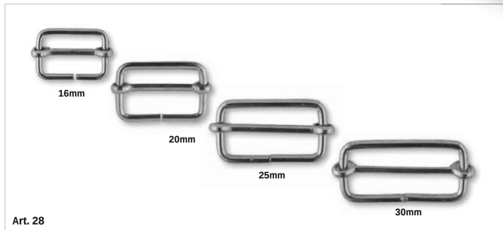
art. 28 FIBBIA passante scorrevole 16x10,5mm 20x12mm 25x13mm 30x13mm 35x14mm 40x14mm 45x18,5mm 50x20mm
